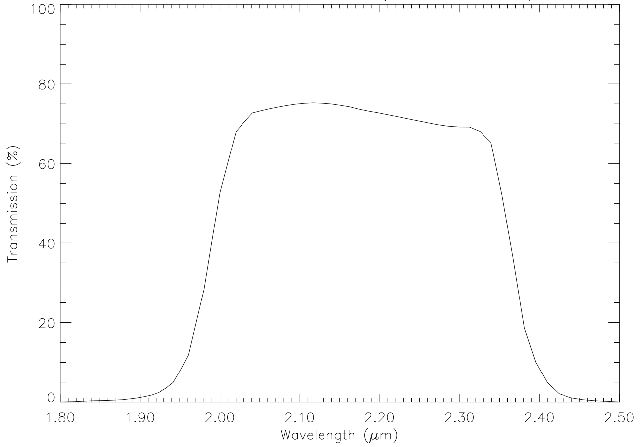
IOTA Filter – K Band, \lambda_c=2.17\mu\text{m} , FWHM= 0.38\mu\text{m}
