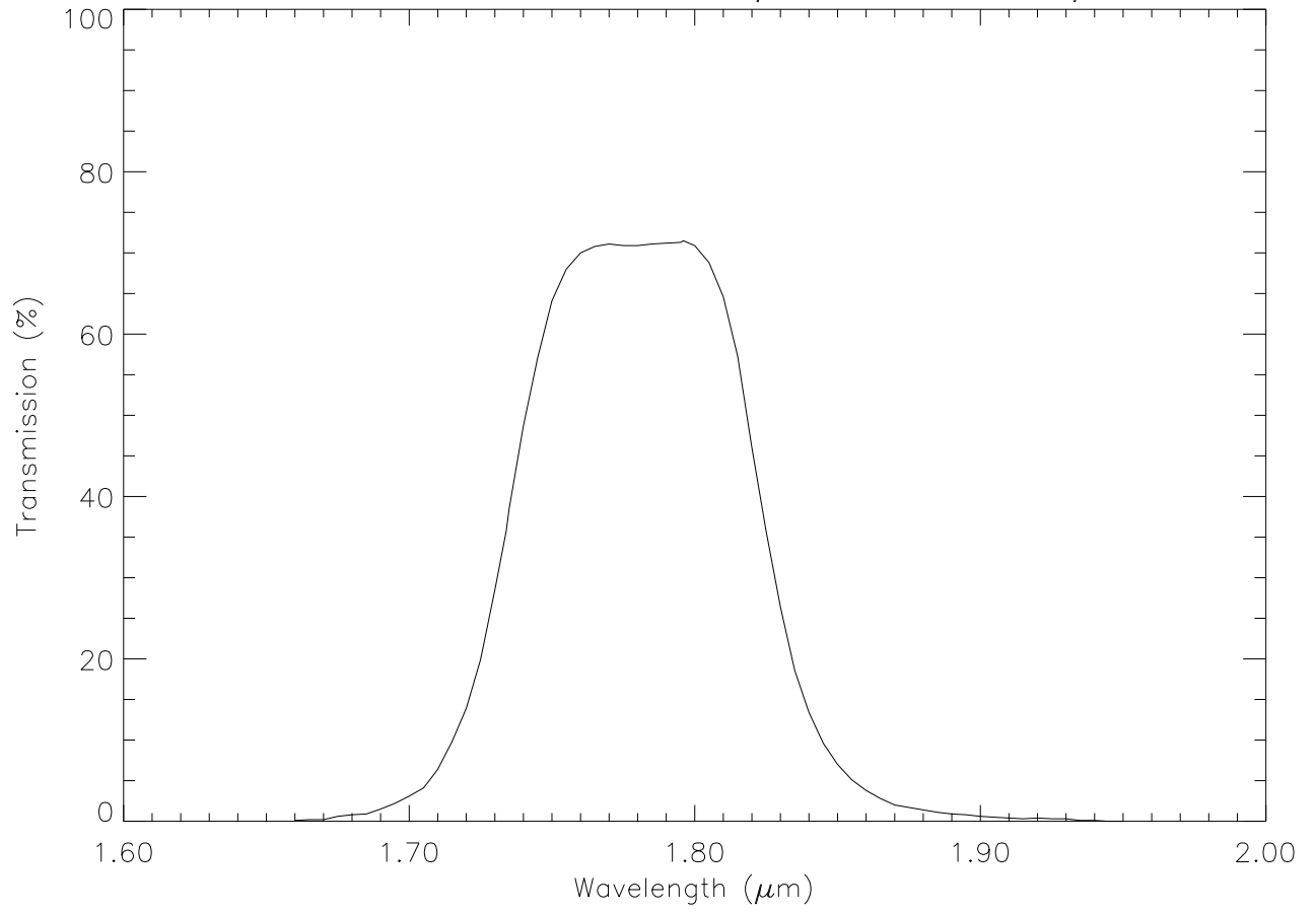
IOTA Filter - H178, \lambda_c=1.78\mu\text{m} , FWHM=0.091 \mu\text{m}
