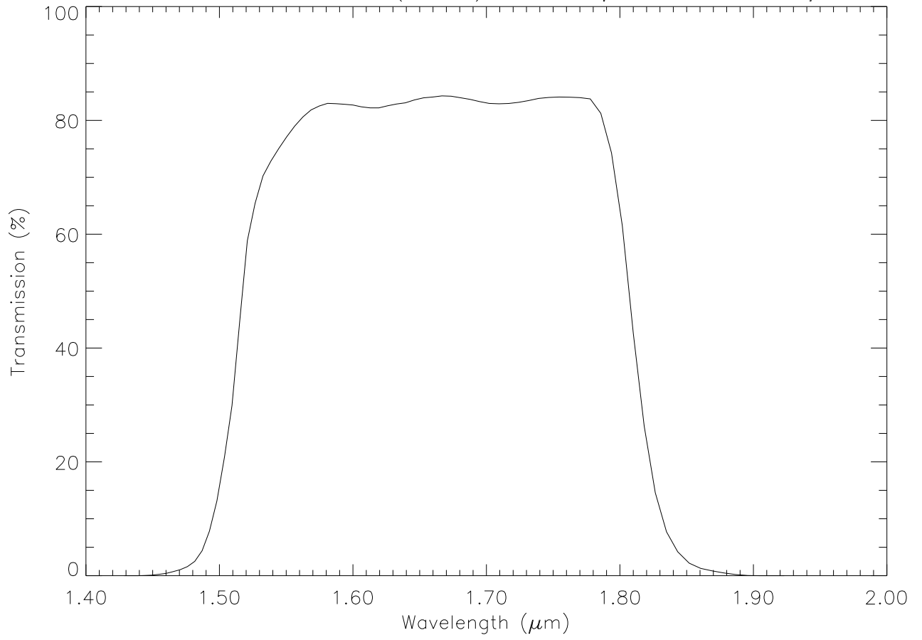
IOTA Filter – H Band (broad), \lambda_c=1.66\mu\text{m} , FWHM= 0.30\mu\text{m}
