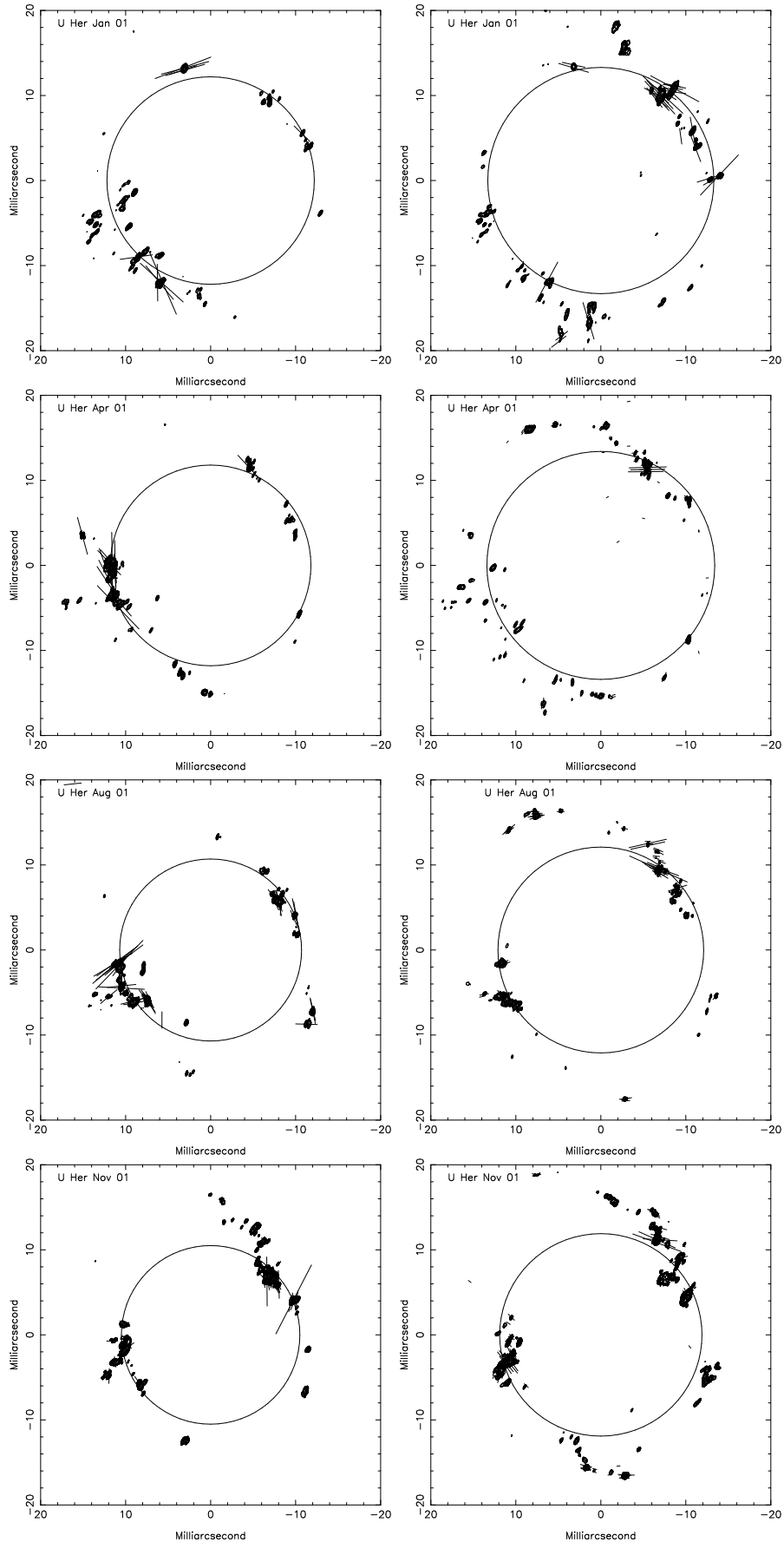
Fig. 8. U Herculis. Left column is \nu=2 , J=1-0 transition of SiO at 42.8 GHz, right column is \nu=1 , J=1-0 transition of SiO at 43.1 GHz. Polarization “E” vectors are over-plotted on contours of total intensity. Circles show the fitted rings as given in Table 2.
