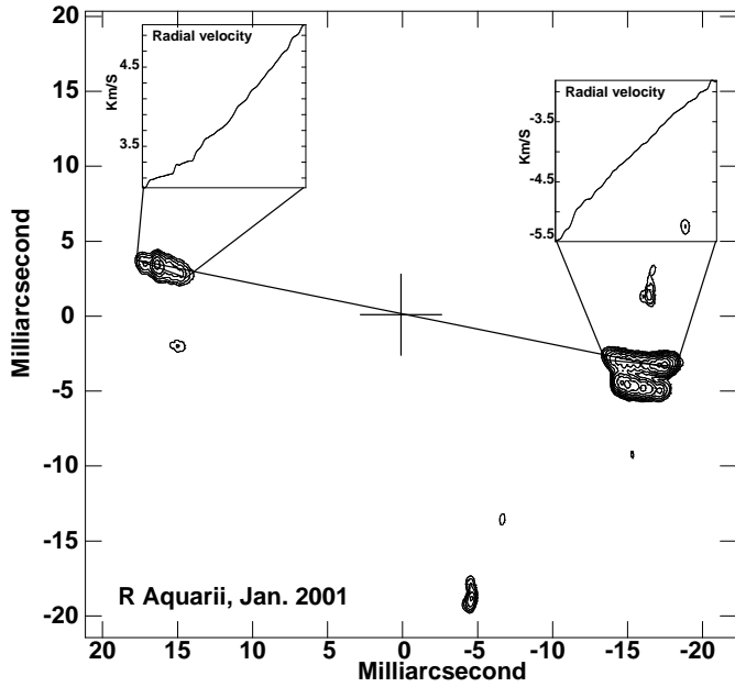
Fig. 14. Total intensity contours of R Aquarii in the \nu=1 , J=1-0 transition in January 2001 with inset plots showing the run of radial velocity in slices through the two extended linear features. Velocities are with respect to the systemic velocity of -24.5 km/s. A cross marks the fitted center of the star and a line connects the extended features on either side.
