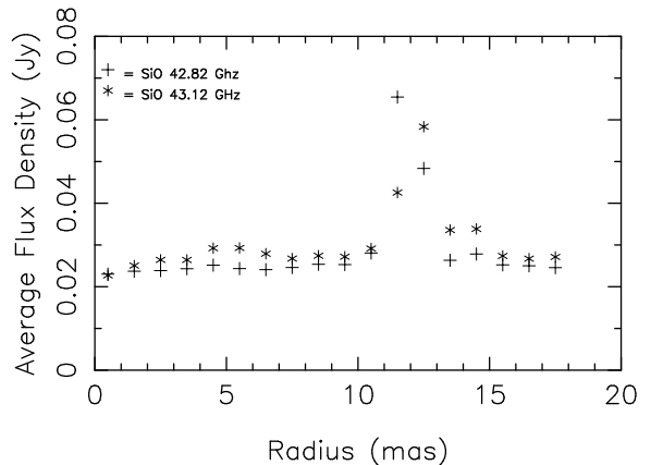
Fig. 1. Stokes' I flux density averages per unit area in annuli around the center of U Orionis demonstrating the concentration of the maser emission into a ring.
