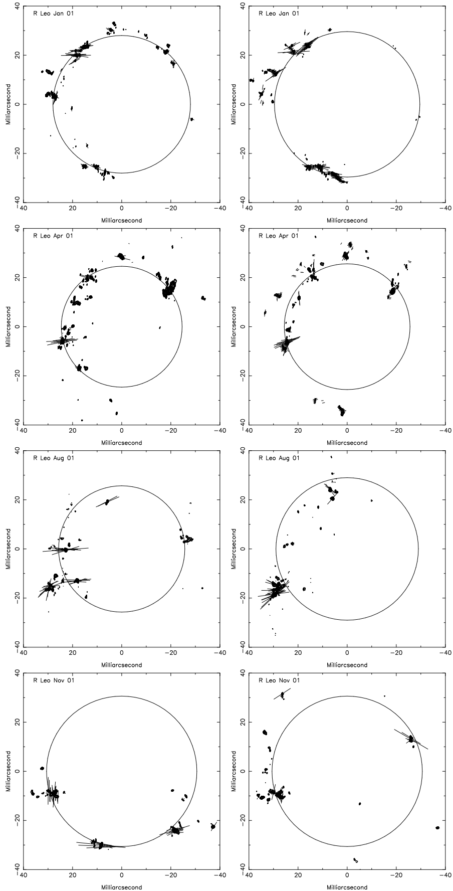
Fig. 5. R Leonis. Left column is \nu=2, J=1-0 transition of SiO at 42.8 GHz, right column is \nu=1, J=1-0 transition of SiO at 43.1 GHz. Polarization “E” vectors are over-plotted on contours of total intensity. Circles show the fitted rings as given in Table 2.
