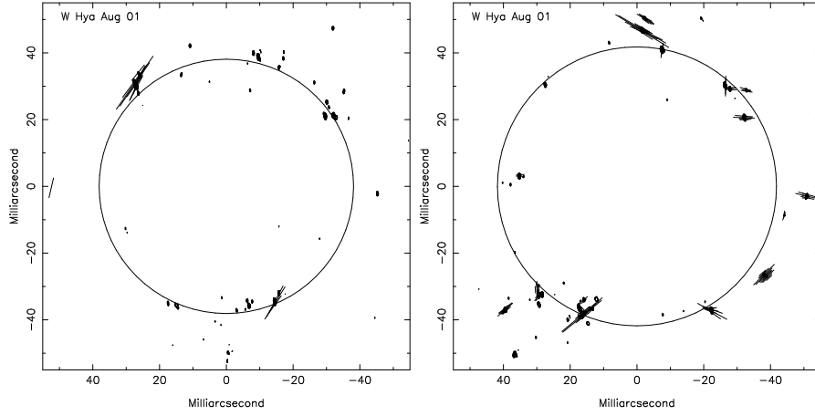
Fig. 6. W Hydrae. Left column is \nu=2 , J=1-0 transition of SiO at 42.8 GHz, right column is \nu=1 , J=1-0 transition of SiO at 43.1 GHz. Polarization “E” vectors are over-plotted on contours of total intensity. Circles show the fitted rings as given in Table 2.
