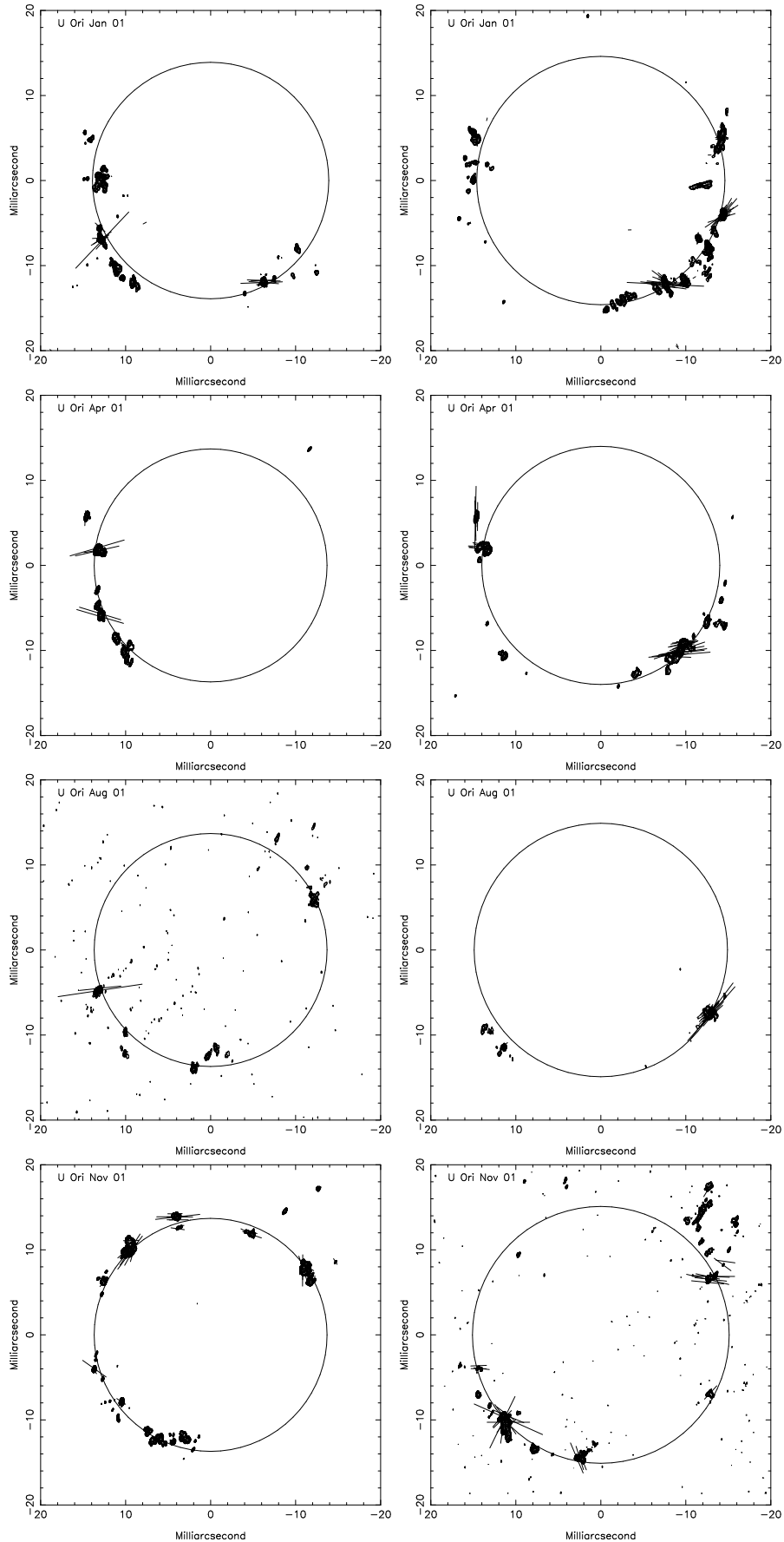
Fig. 4. U Orionis Left column is \nu=2 , J=1-0 transition of SiO at 42.8 GHz, right column is \nu=1 , J=1-0 transition of SiO at 43.1 GHz. Polarization “E” vectors are over-plotted on contours of total intensity. Circles show the fitted rings as given in Table 2.
