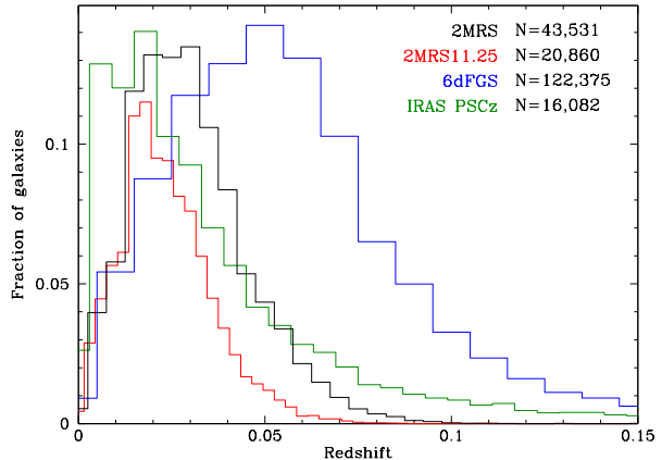
FIG. 6.— Distribution of galaxies as a function of redshift for 2MRS and for some of the redshift surveys listed in Table 1.
